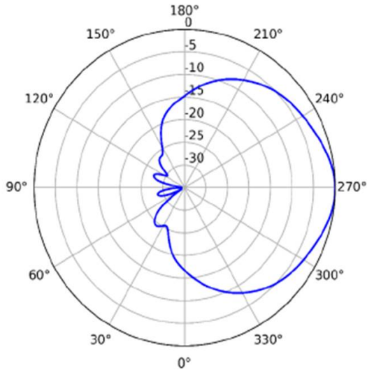
2.4GHz (Horizontal)
